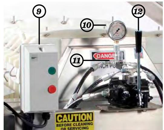
Fig 1.2: Switch and Valve Assembly
